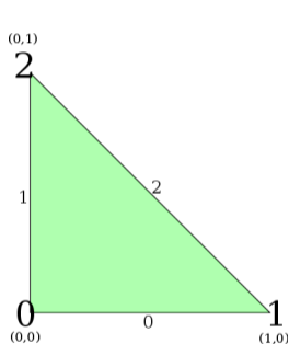
simplex 2D
