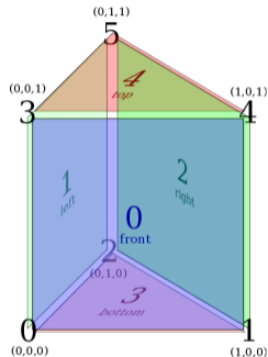
prism
