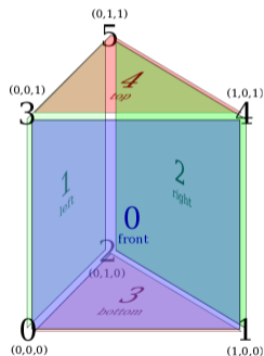
prism
