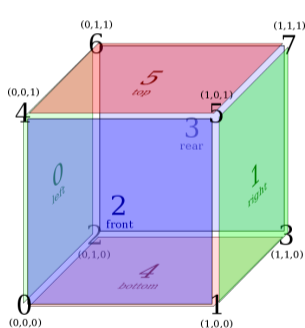
cube 3D
