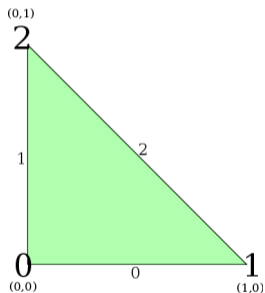
simplex 2D
