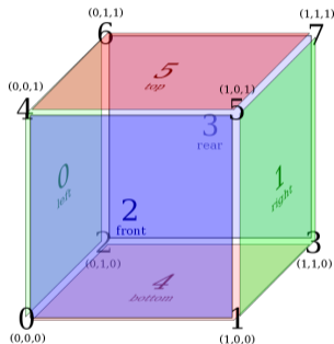
cube 3D
